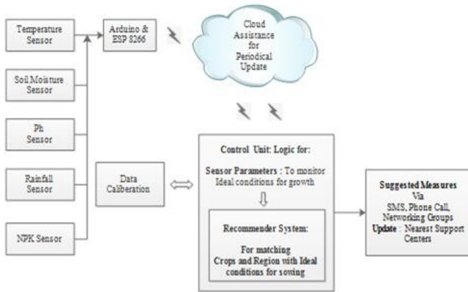
Fig. 6. Generalized block diagram of proposed platform
