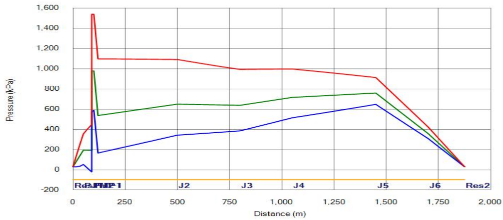
Fig. 10. Pressures (max, min and initial) for transient state along the protected irrigation pipeline system
