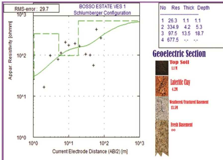
Fig. 3. A KA curve type obtained from VES 1
