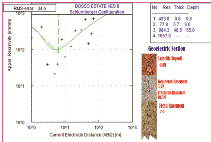
Fig. 4. Example of an H curve type
