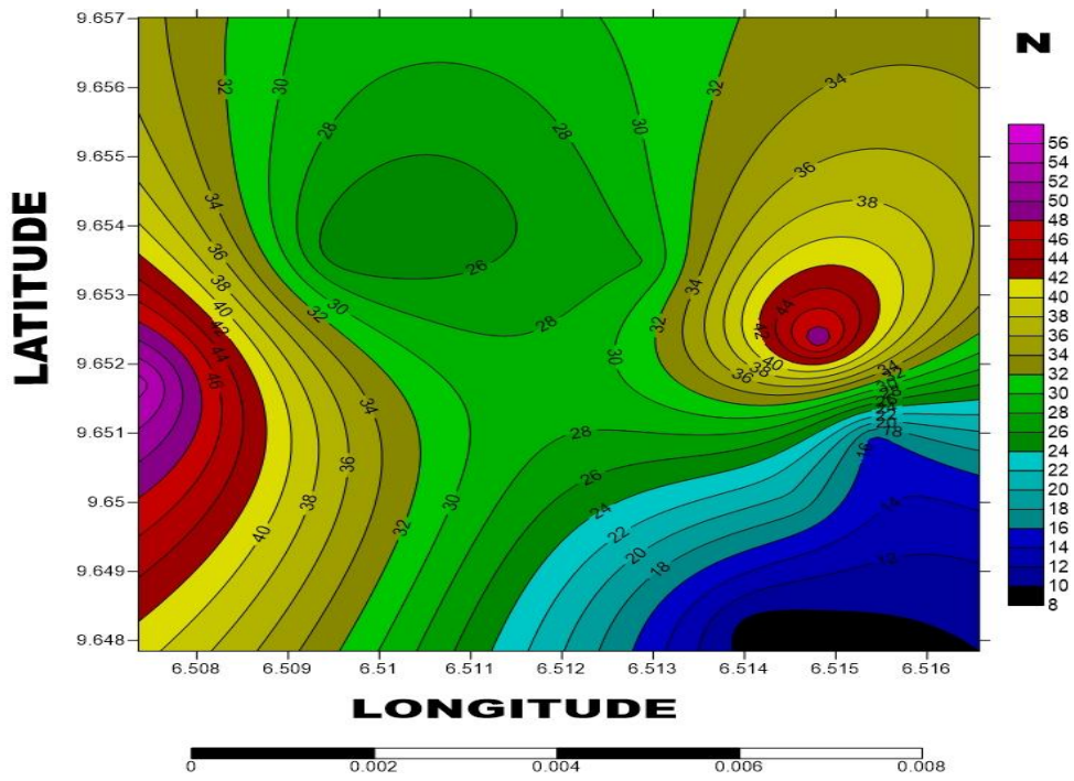
Fig. 7. Aquifer thickness contour map of part of Bosso Estate
