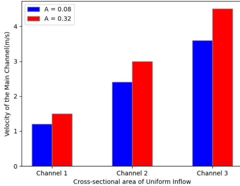
Effect of Variation of Cross-Sectional Area on the Velocity of Main Channel
