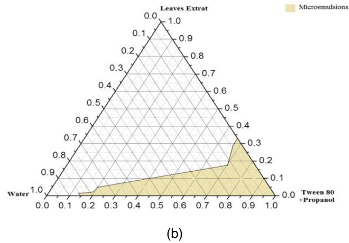
Fig. 5. (a) Ternary Phase diagram of system: Water/ seeds oil / Tween 80: propanol (2:1) at 25°C. The microemulsion region is represented by beige color. (b):Ternary Phase diagram of system: Water/ leaves extract / Tween 80: propanol (2:1) at 25°C. The microemulsion region is represented by beige color.
