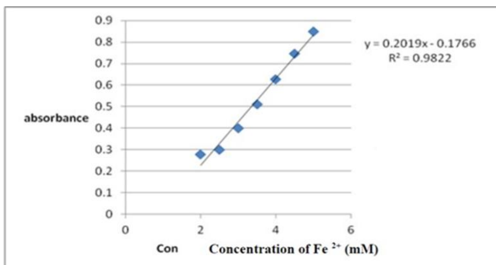
Fig. 8. Calibration curve of Fe +2 standard used for FRAP study
