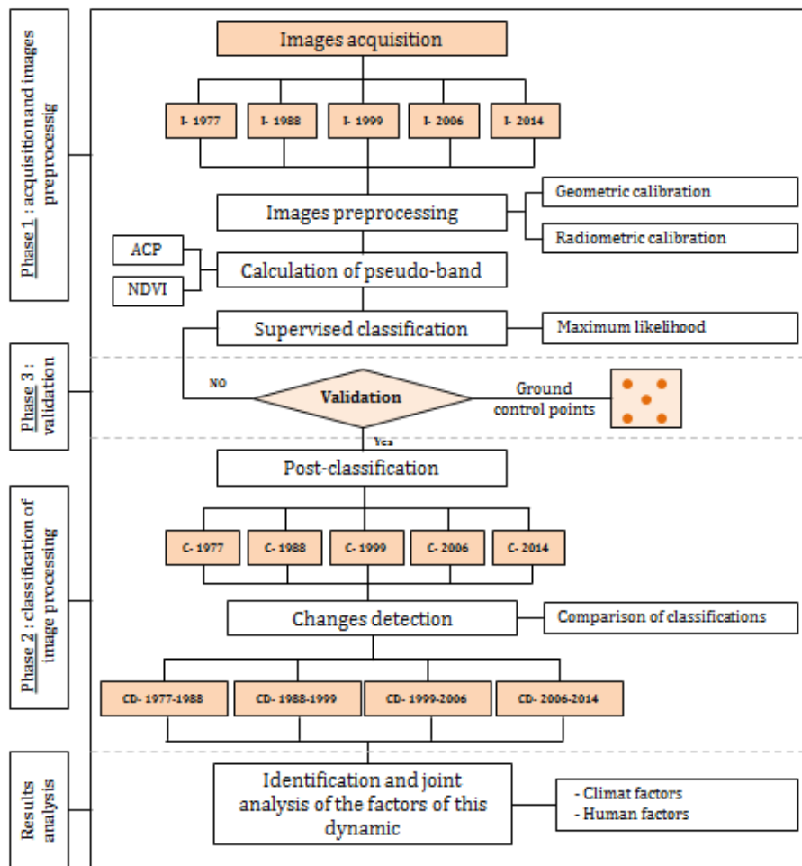
Fig. 2. Flowchart of the methodology of processing and analysis of Landsat images
