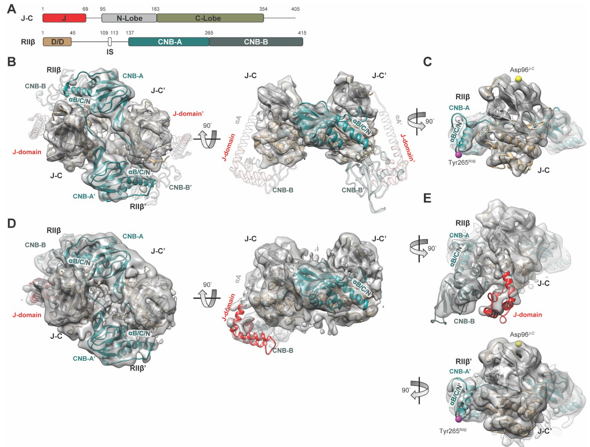
Fig 1. Cryo-EM structure of the RII \beta 2 J-C 2 holoenzyme. (A) Domain diagram and color coding of RII \beta 2 J-C 2 holoenzyme. (B, C) Cryo-EM structure the RII \beta 2 J-C 2 holoenzyme (PDB = 6WJG) at 6Å with C2 symmetry imposed. (C) The EM density of the RII \beta 2 J-C 2 holoenzyme starts at Asp96 J-C (equivalent to Asp41 C in the WT C subunit) in the N-terminus of the J-C subunits and ends at Tyr265 RII \beta in the RII \beta subunit. The density for the A-helix, J-domain, and CNB-B domains are missing. (D, E) Structure of the RII \beta 2 J-C 2 holoenzyme structure (PDB = 6WJF) after classification reveals presence of ordered J-domain and CNB-B domain. (E) One of the protomers of RII \beta 2 J-C 2 holoenzyme has ordered J-domain and CNB-B domain, whereas J-domain, A-helix, and CNB-B domain are flexible in the other protomer. CNB, cyclic nucleotide binding; cryo-EM, cryo-electron microscopy; PDB, Protein Data Bank; WT, wild-type.
