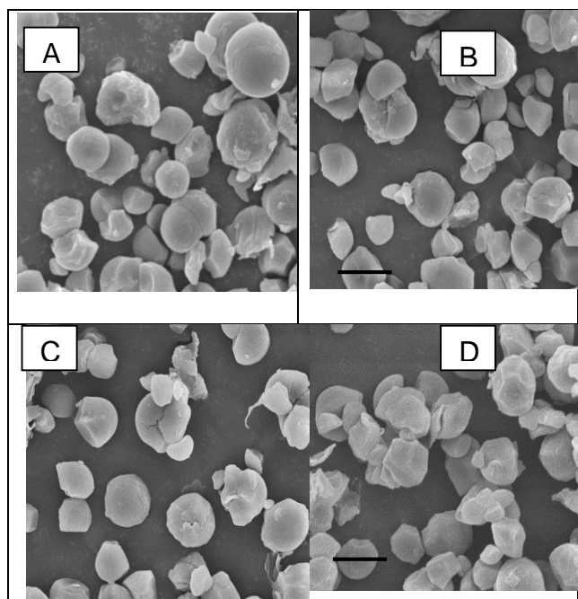
Fig. 1. Scanning electron micrographs (SEM) of native and cross-linked breadfruit starches ( 10 µm). Where A: Native breadfruit starch; B, C & D: CLBS with 2%, 5%, and 10% STMP/STPP, respectively.
