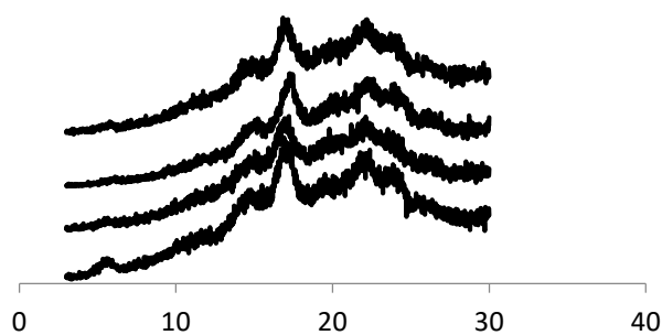
Fig. 2. X-ray diffractograms of native and CLBS. Where NBS: native breadfruit starch and CLBS-2, CLBS-5, and CLBS-10: cross-linked breadfruit starches with 2%, 5% and 10% STMP/STPP, respectively.
